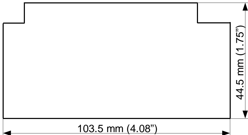
Fig. 1 Dimensions of GPS125
